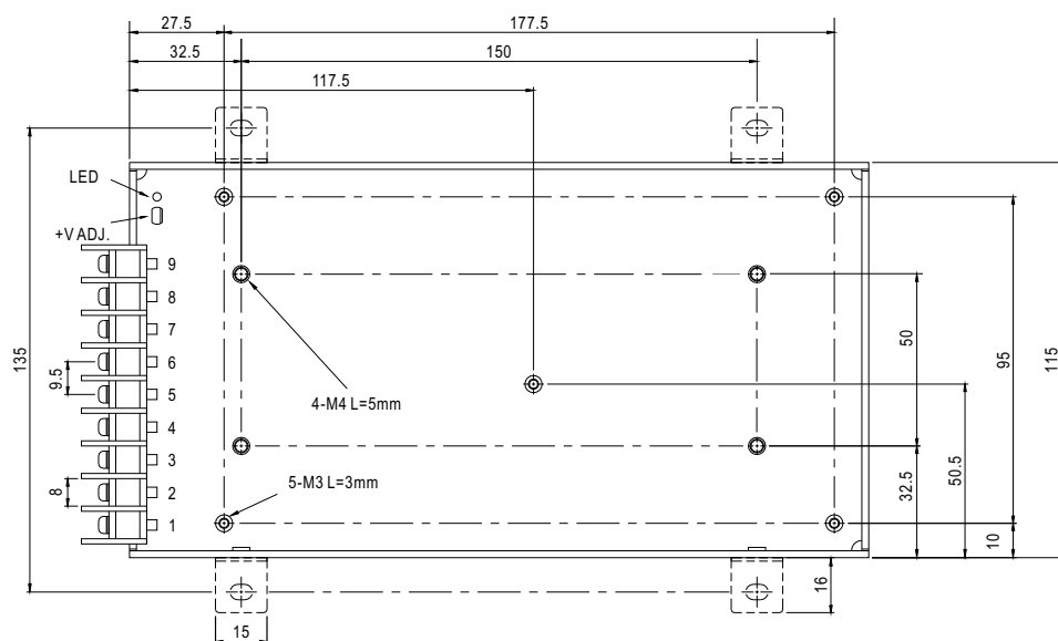
Terminal pin number assignment:
