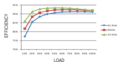
RSD-300D-5
