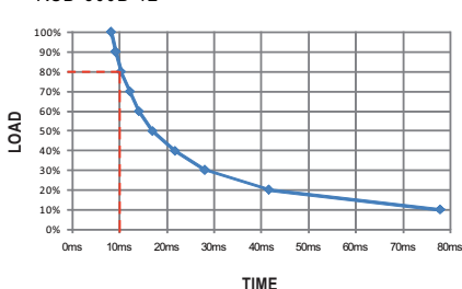
RSD-300B-12
