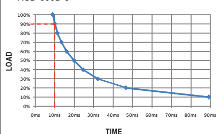
RSD-300B-5
