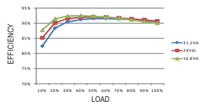
RSD-300C-12
