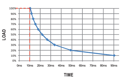
RSD-300C-5
