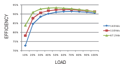
RSD-300D-48
