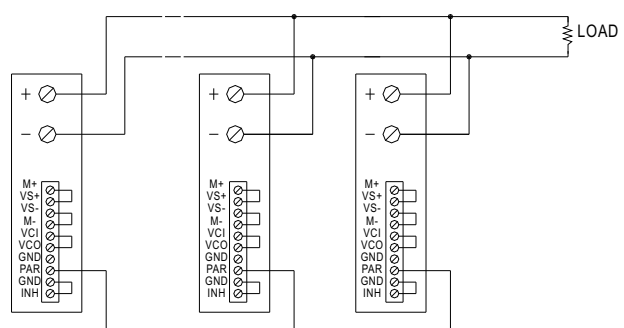
PARALLEL OPERATION
